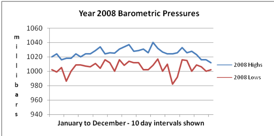
Figure 2: Year 2008 Barometric pressures
